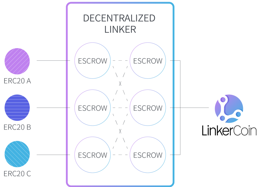
FIGURE 3) DECENTRALIZED LINKER 1
