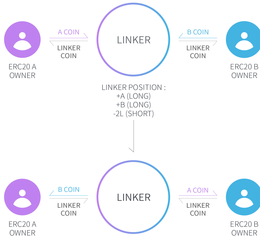
FIGURE 4) DECENTRALIZED LINKER 2
